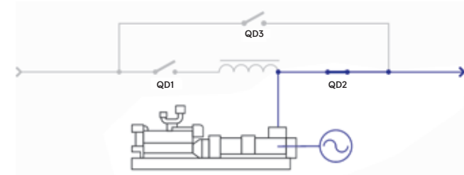
Independent Mode mtu Kinetic PowerPack provides energy as secondary power source, without interruption
