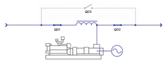
Conditioning Mode mtu Kinetic PowerPack protects the load
